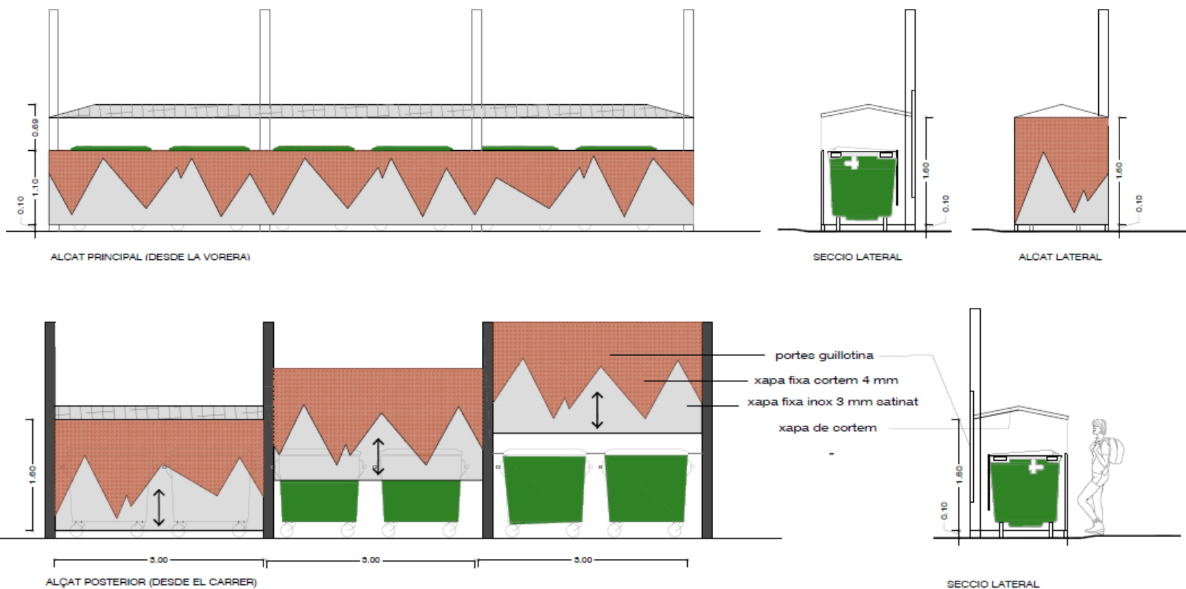
DETALL RECINTE ESCOMBRARIES (fase 1) E:1/50
